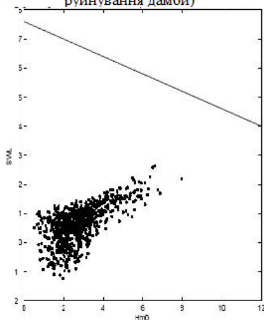
Figure 1. Wave height H_{m0} and sea level SWL recorded during 828 storm events for the Dutch Coast. The area above the solid line represents a possible failure area.
